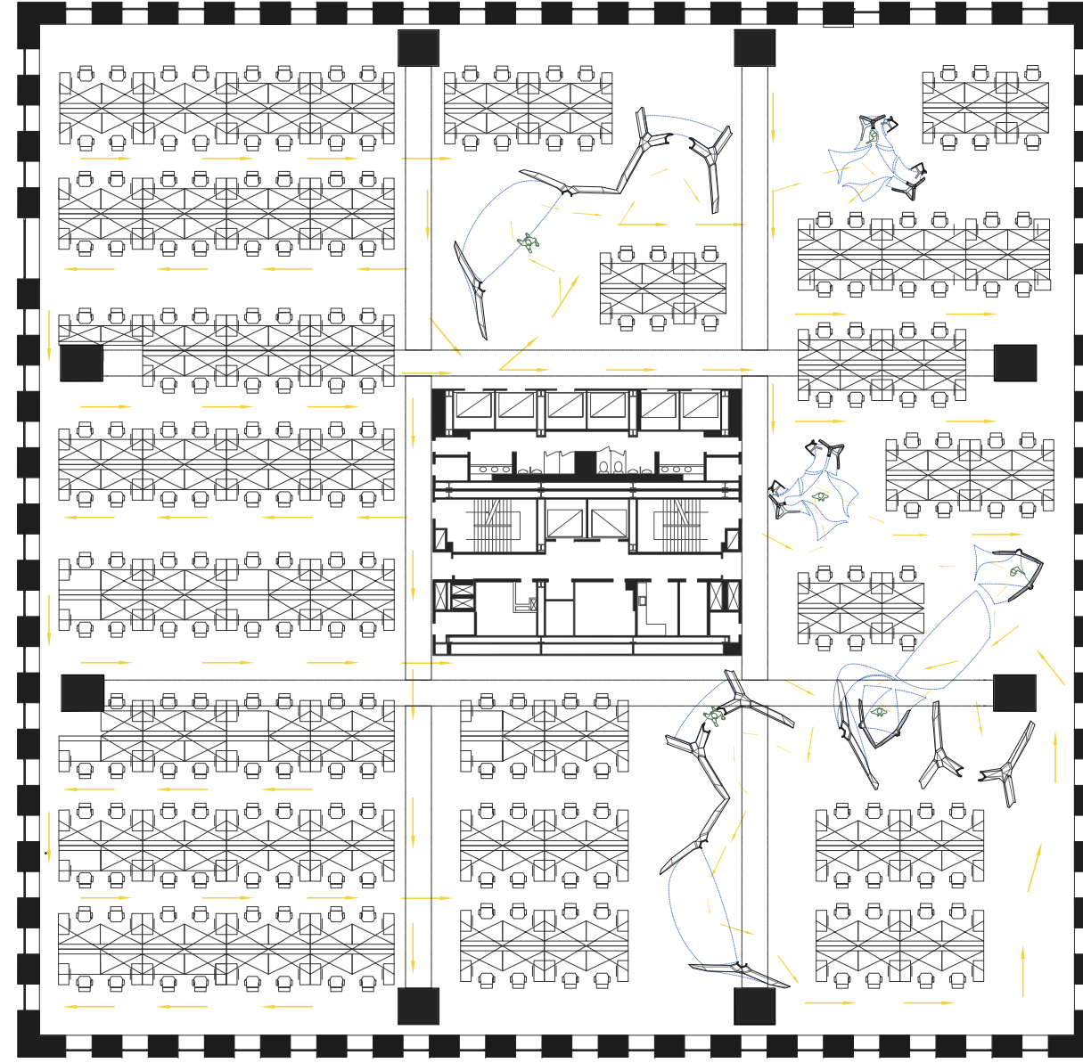
dynamic partitions
