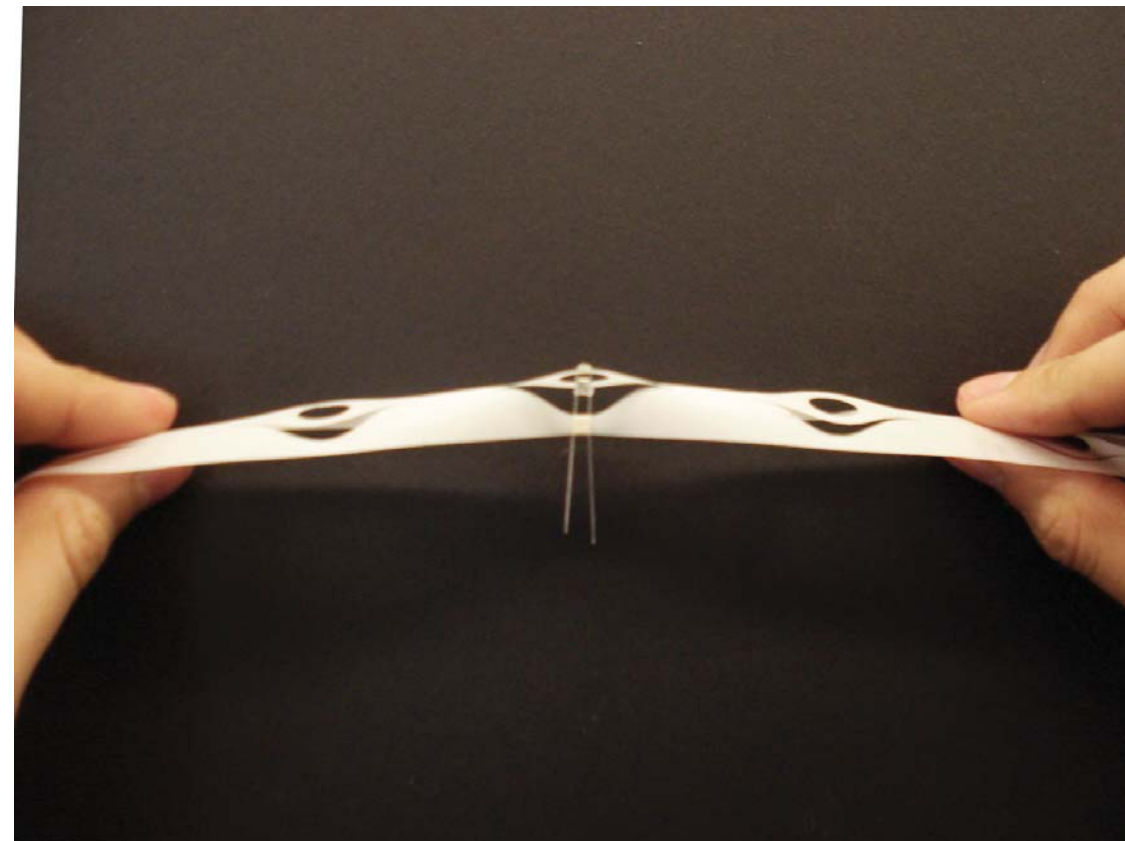
INSERT LED AROUND PINCHED SIDES
