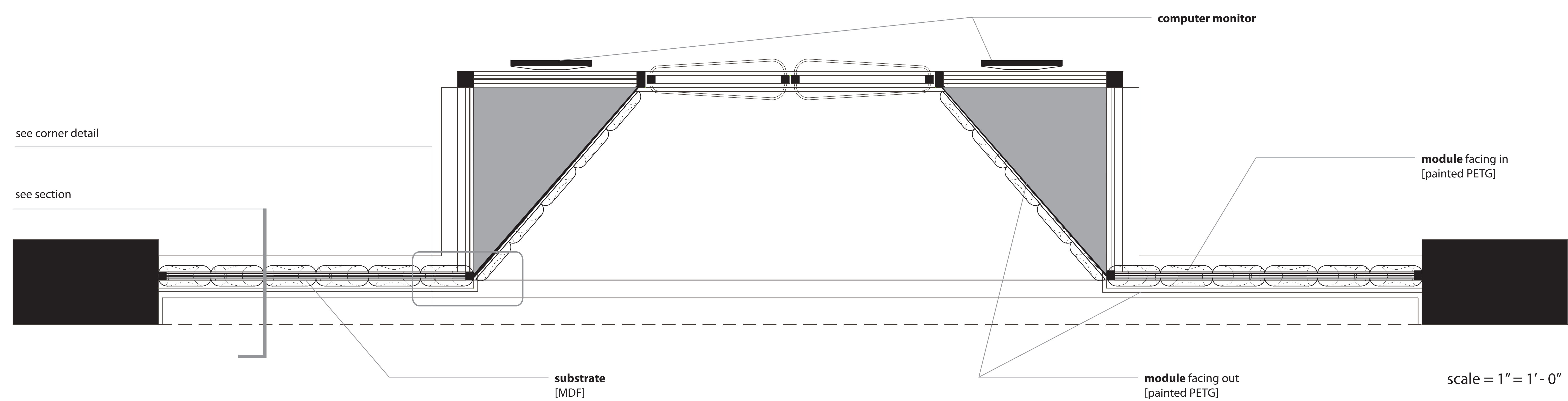
assembly sequence
