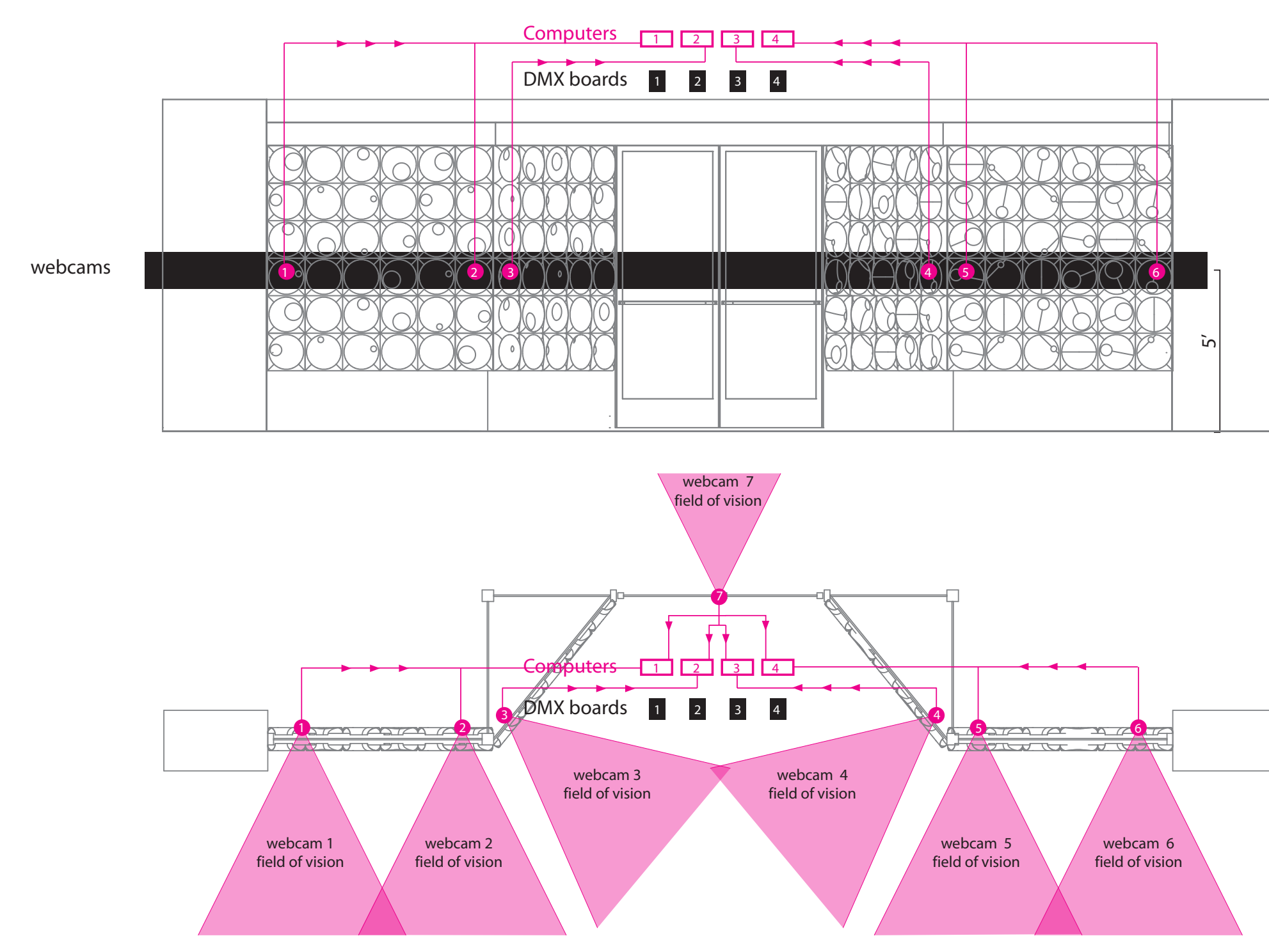
INPUT DIAGRAM
