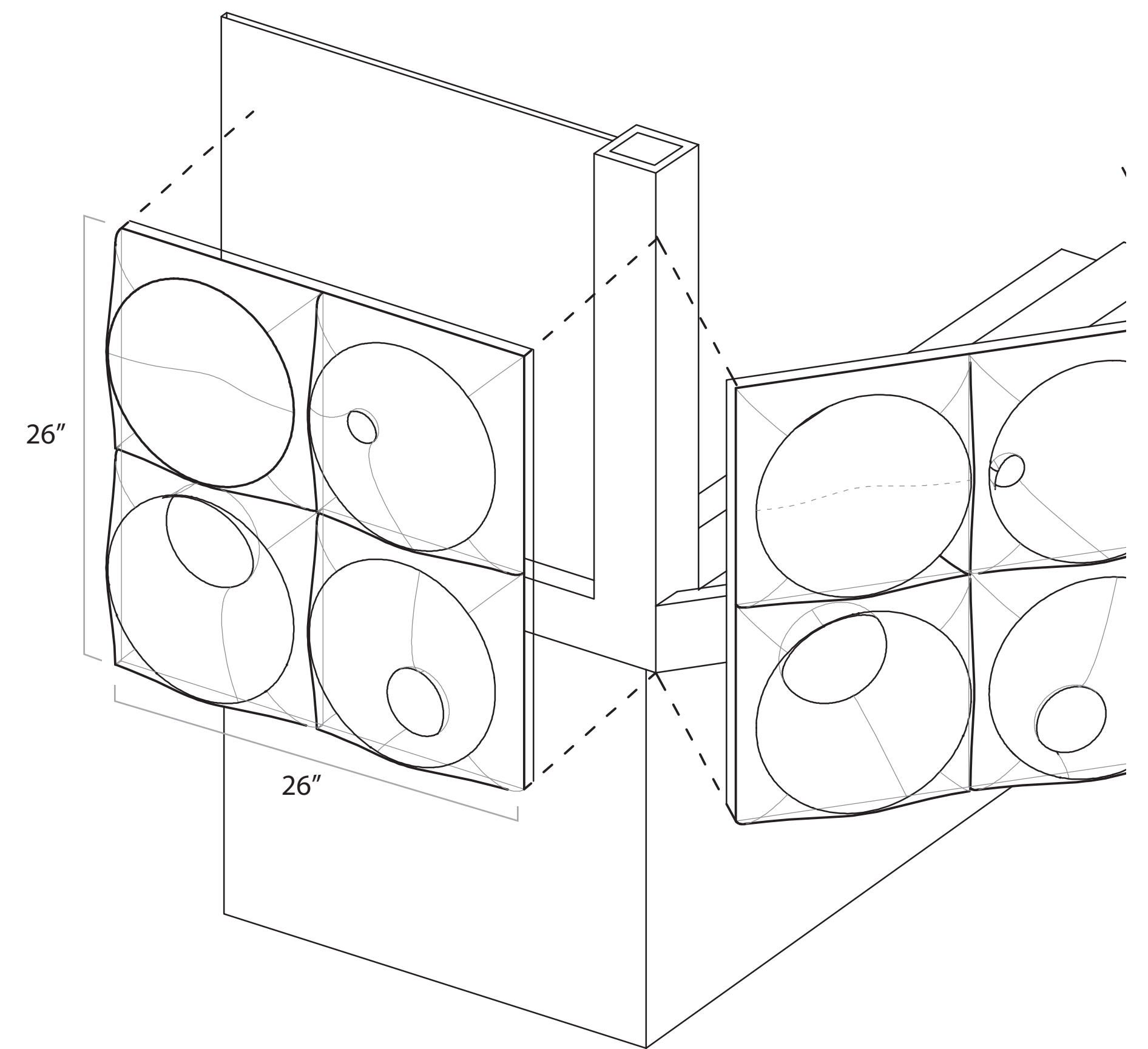
CORNER DETAIL
