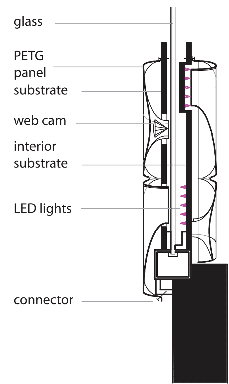
PANEL SECTION
